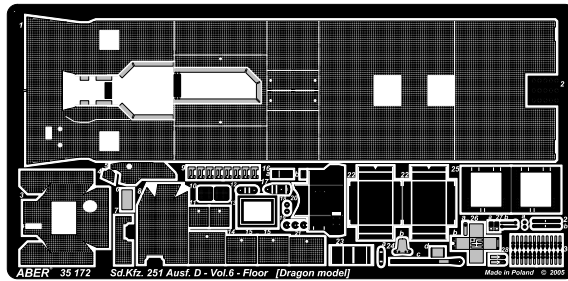
ABER 35 172 Sd.Kfz. 251 Ausf. D - Vol.6 - Floor (Dragon model) Made in Poland © 2005
