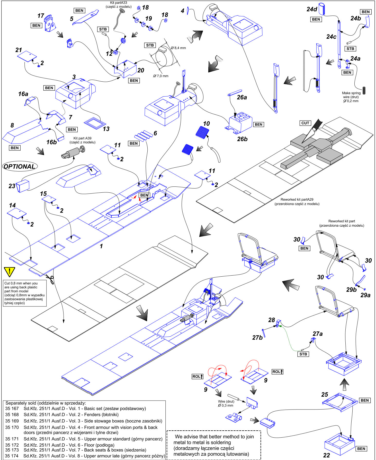
ABER 35 172 Sd.Kfz. 251 Ausf. D - Vol.6 - Floor (Dragon model) Made in Poland © 2005
